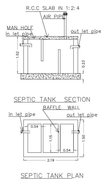
SEPTIC TANK PLAN
