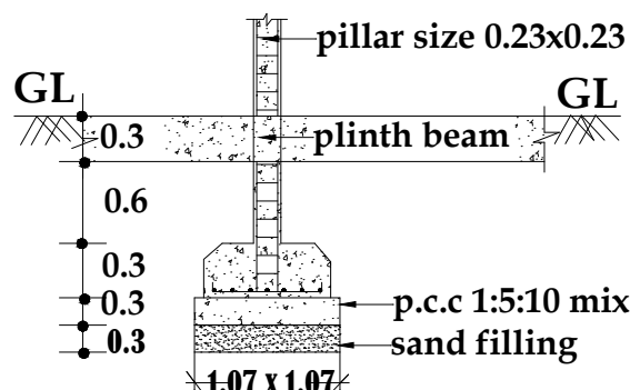
FOUNDATION DETAILS
