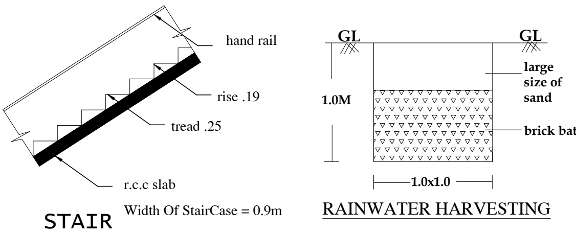
STAIR
