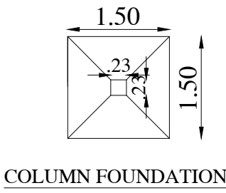
COLUMN FOUNDATION
