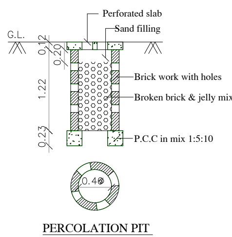
PERCOLATION PIT
