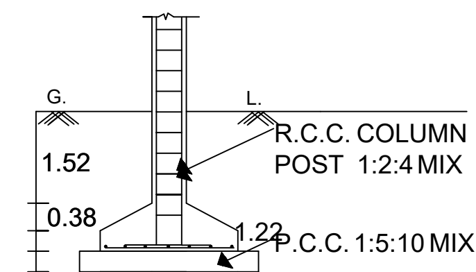
FOUNDATION DETAILS
