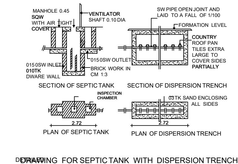
DRAWING FOR SEPTIC TANK WITH DISPERSION TRENCH
