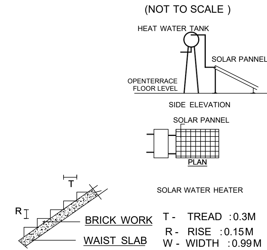
STAIRCASE DETAILS
