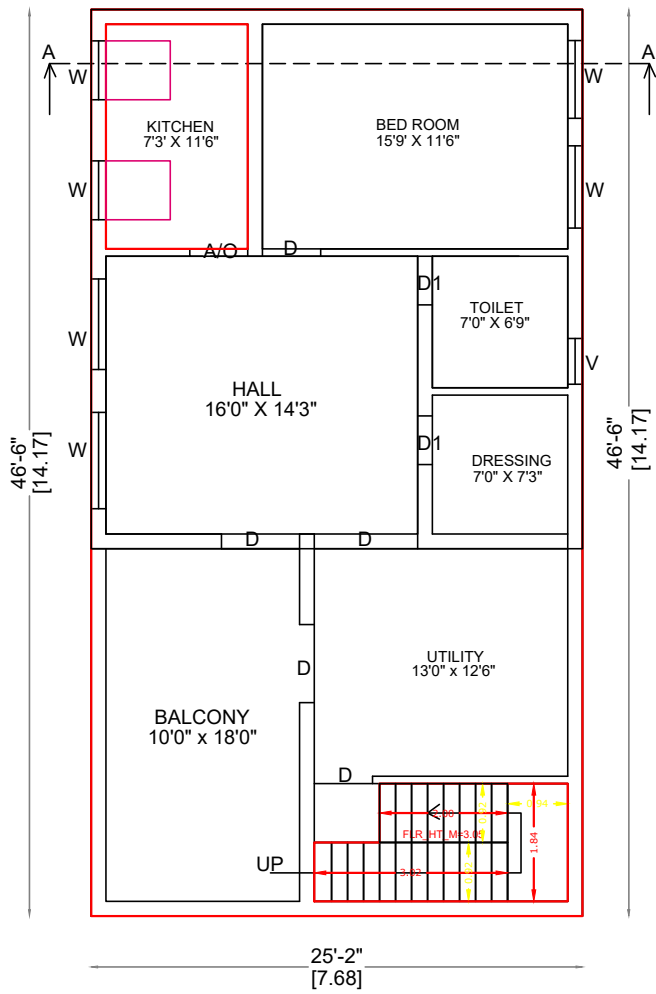
EXG.,FIRST FLOOR PLAN
