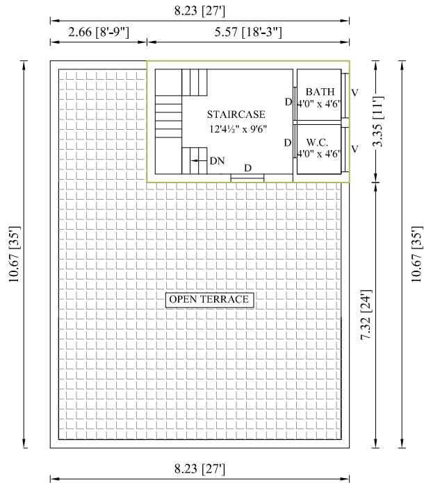
HEAD ROOM & OPEN TERRACE PLAN
