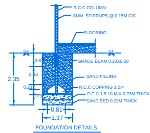
FOUNDATION DETAILS
