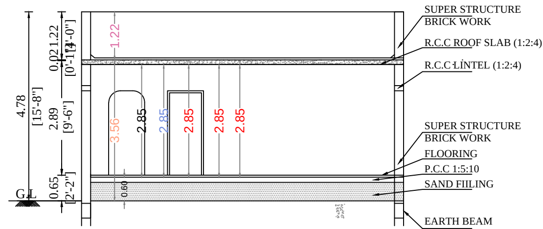
SECTION X - X
