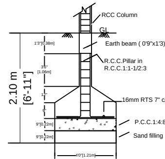
FOUNDATION DETAILS
