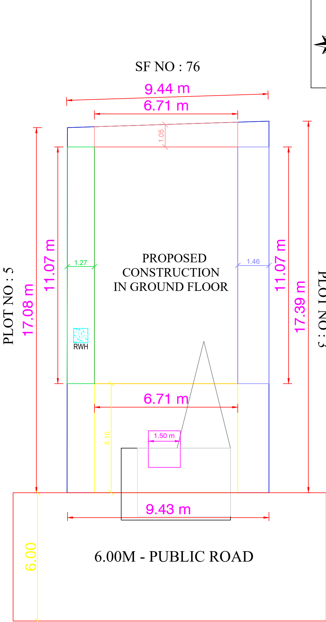
SITE PLAN
