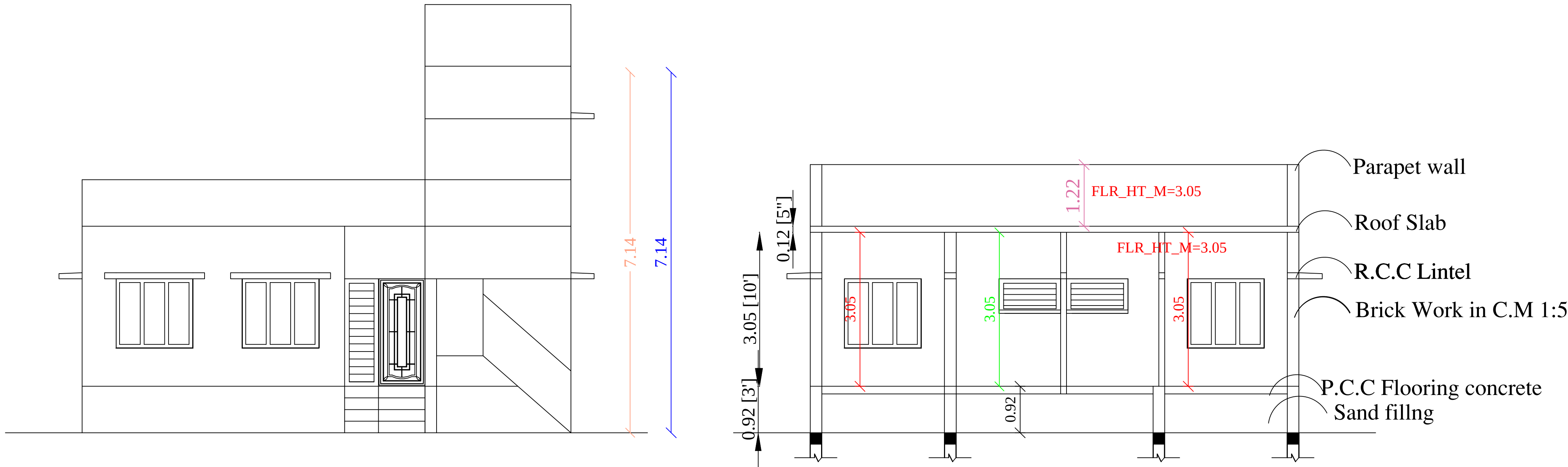
FRONT ELEVATION
