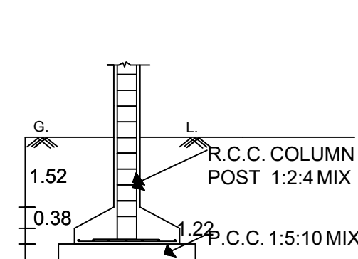
FOUNDATION DETAILS
