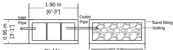
PLAN
