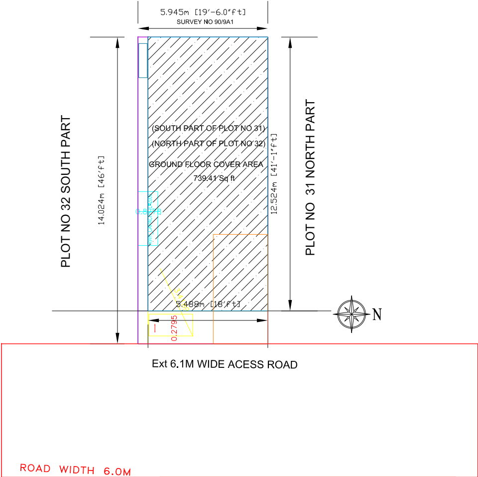
SITE LAYOUT PLAN
