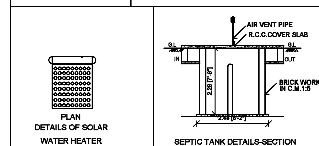
SEPTIC TANK DETAILS-SECTION
