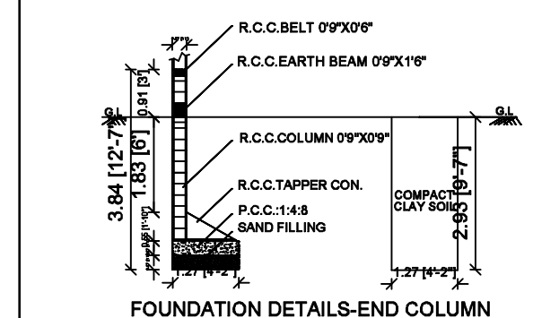
FOUNDATION DETAILS-END COLUMN
