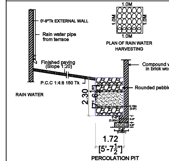
PERCOLATION PIT
