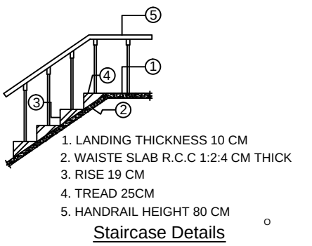
Staircase Details
