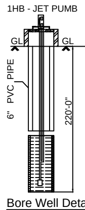
Bore Well Details
