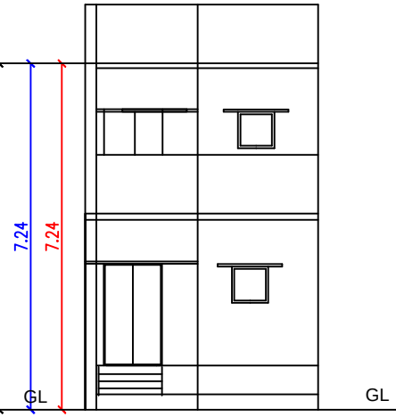
FRONT ELEVATION
