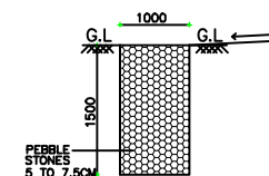
SECTION OF PEBBLE TRENCH SCALE : 1: = 100
