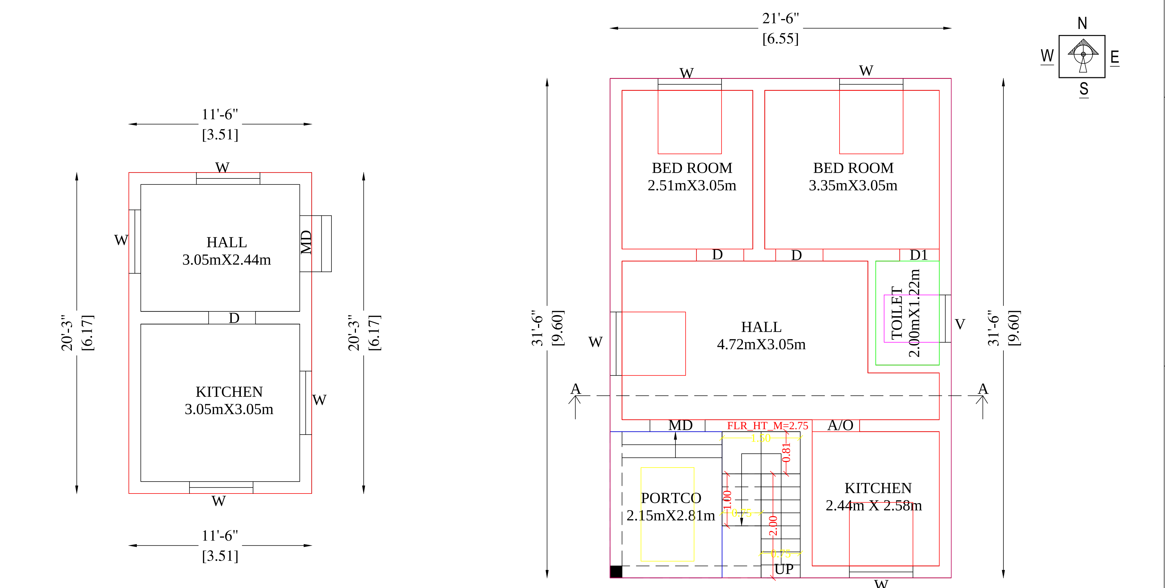
EXG.GROUND FLOOR PLAN
