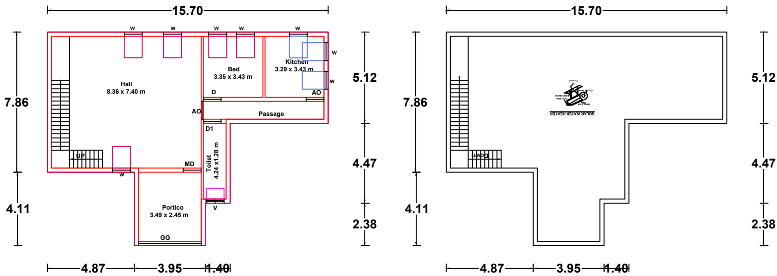
GROUND FLOOR
