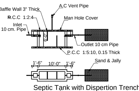
Septic Tank with Dispersion Trench
