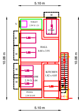
PRO.FIRST FLOOR PLAN
