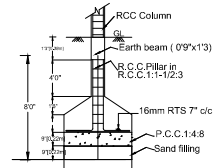
FOUNDATION DETAILS
