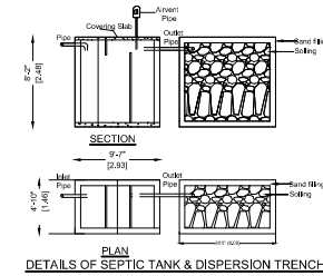
DETAILS OF SEPTIC TANK & DISPERSION TRENCH
