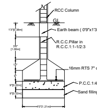
FOUNDATION DETAILS
