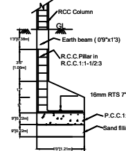
FOUNDATION DETAILS
