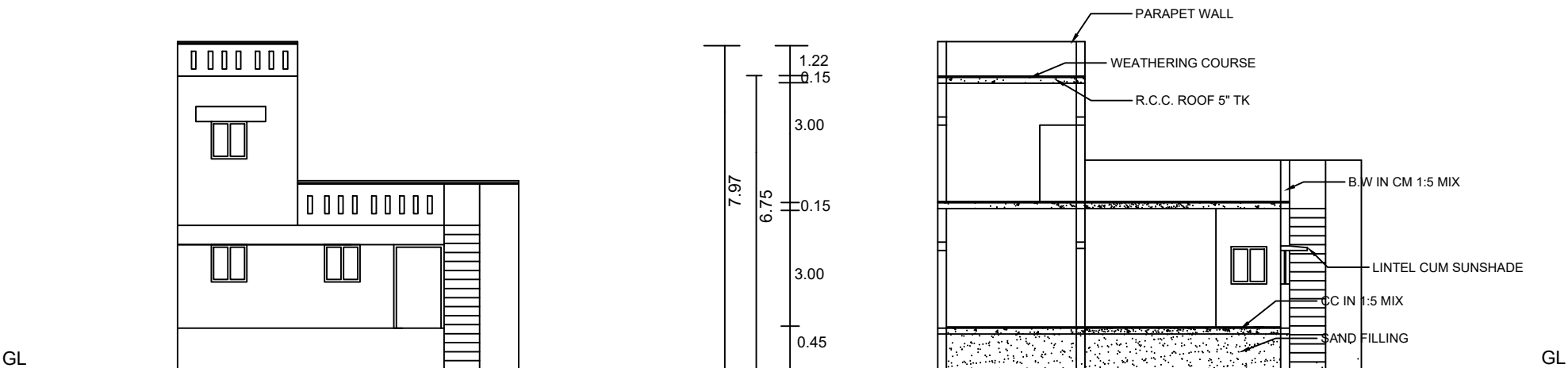
FRONT ELEVATION
