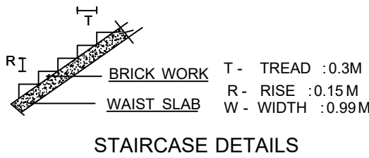
STAIRCASE DETAILS
