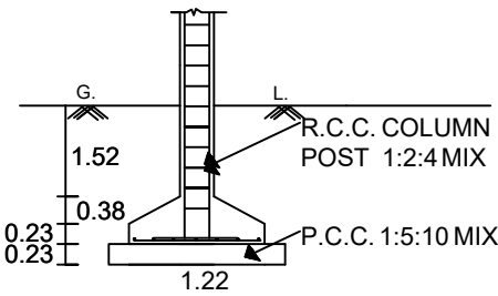
FOUNDATION DETAILS
