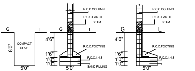
FOUNDATION DETAILS
