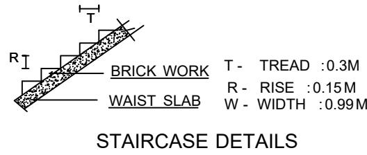
STAIRCASE DETAILS
