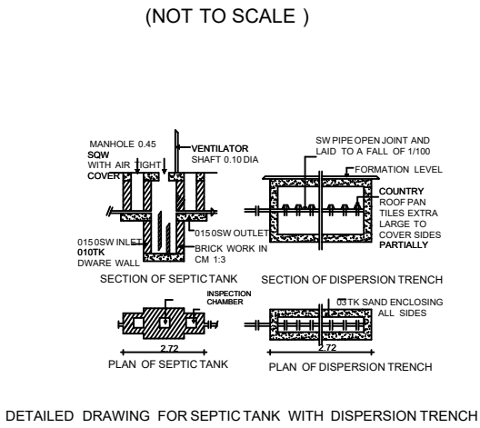
DETAILED DRAWING FOR SEPTIC TANK WITH DISPERSION TRENCH
