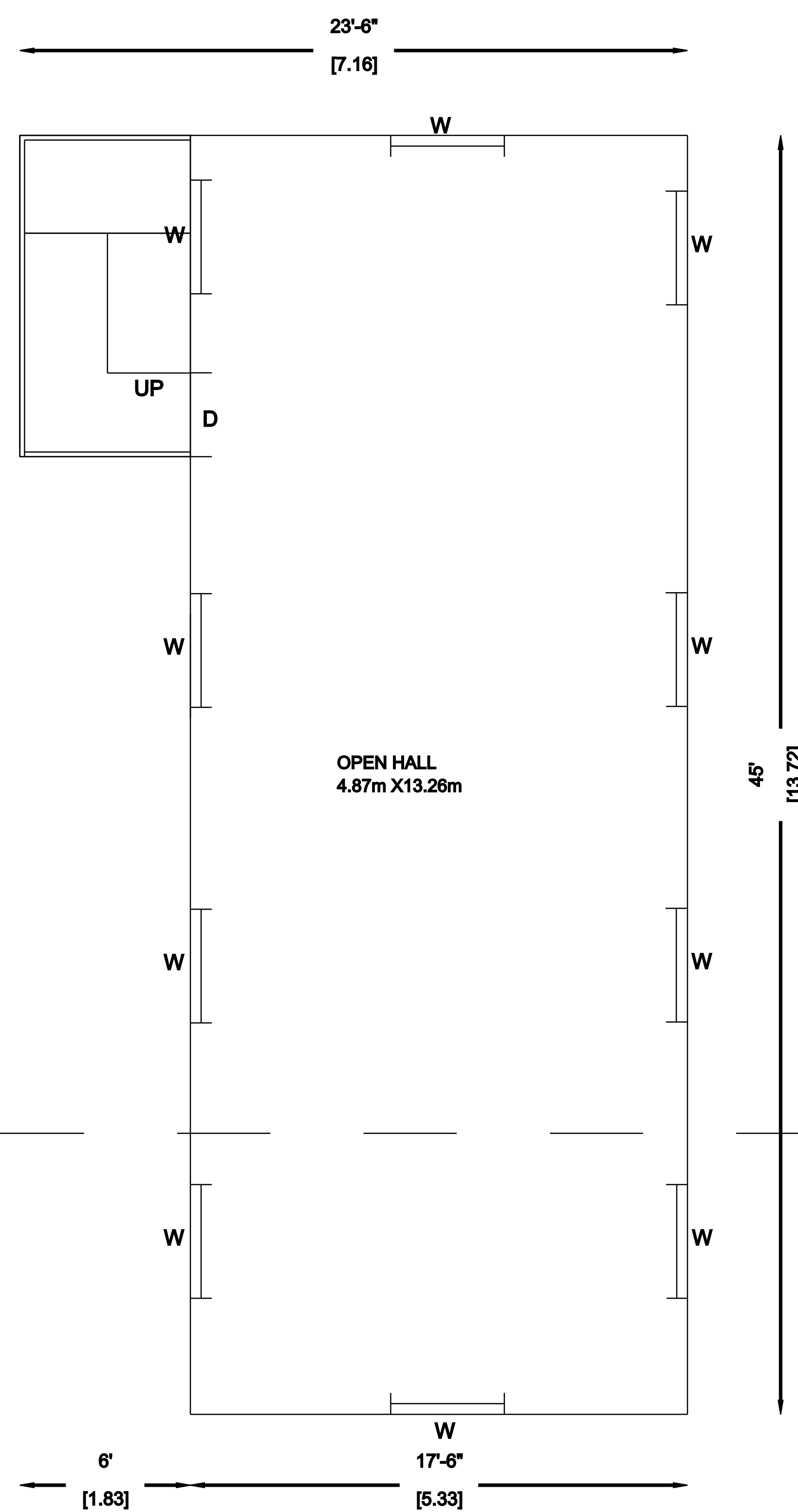
PRO.FIRST FLOOR PLAN
