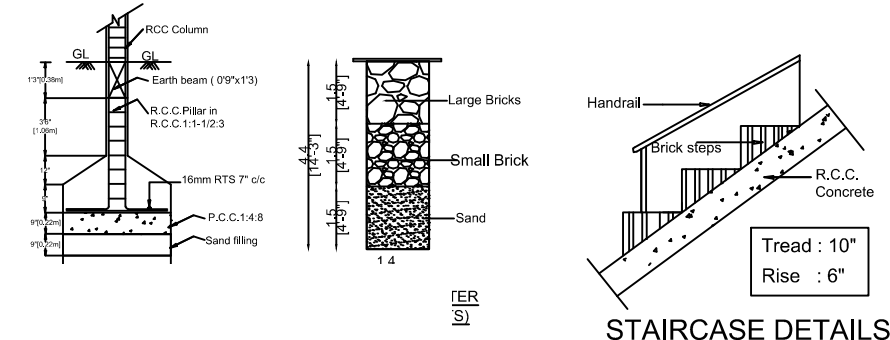
STAIRCASE DETAILS
