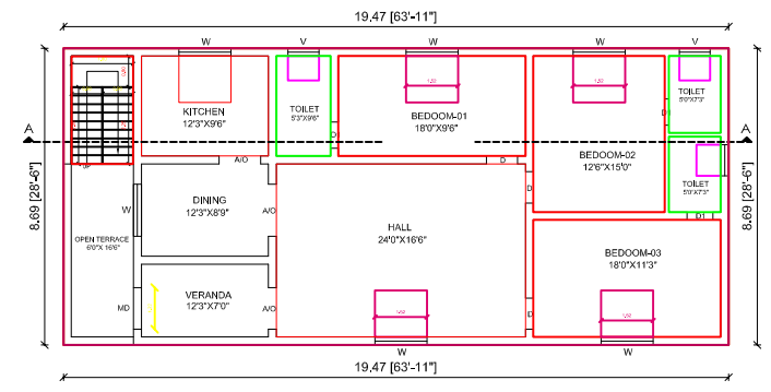
PRO.SECOND FLOOR PLAN
