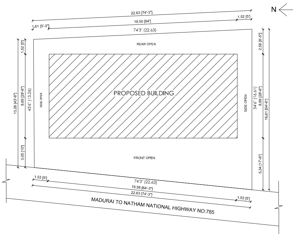
SITE PLAN
