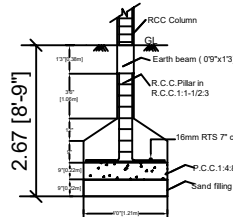
FOUNDATION DETAILS
