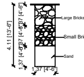
SECTION OF RAIN WATER COLLECTION PITS (INTS.)
