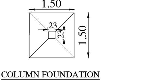
COLUMN FOUNDATION
