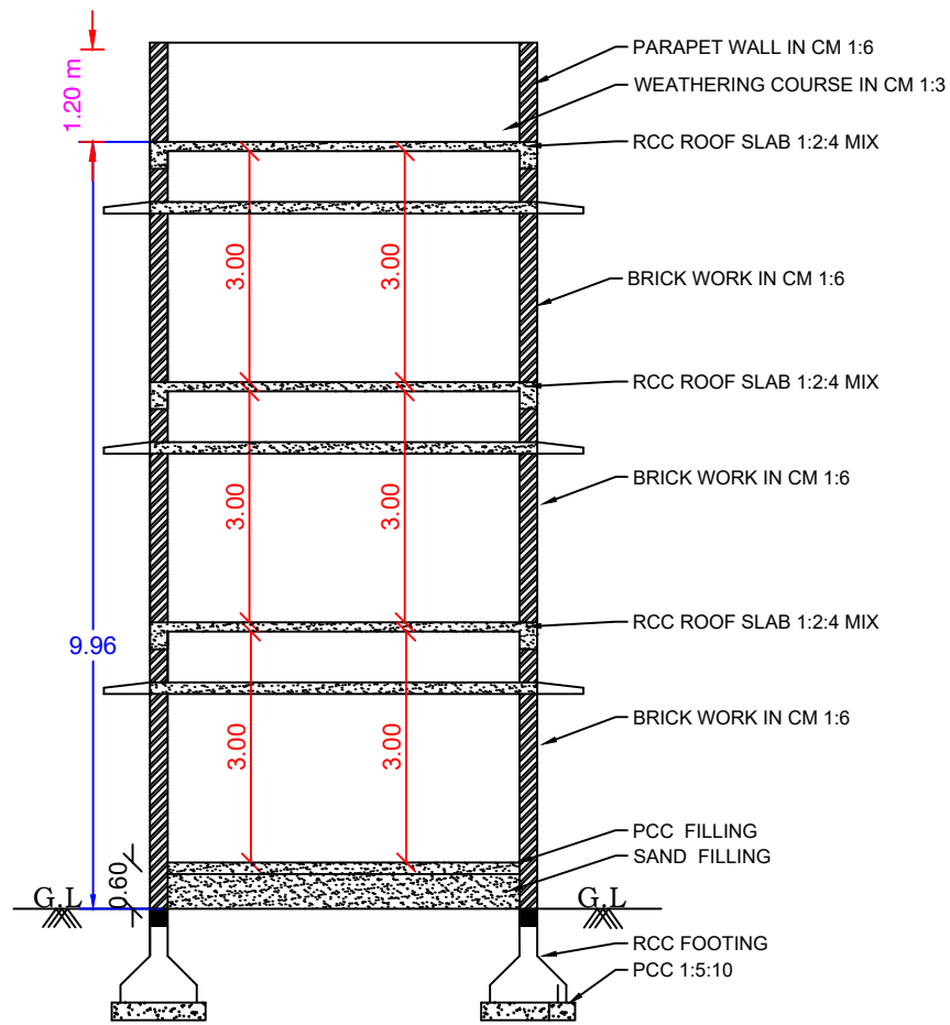
SECTION AB
