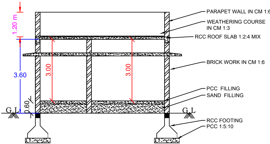
SECTION AB
