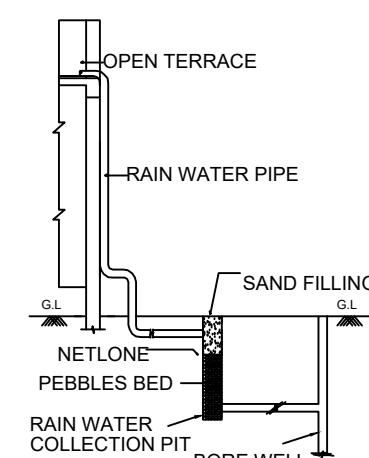
RAIN WATER
