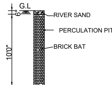
PERCULATION PIT
