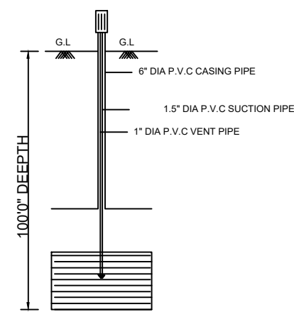
BORE WELL
