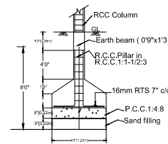
FOUNDATION DETAILS
