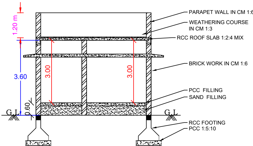
SECTION AB
