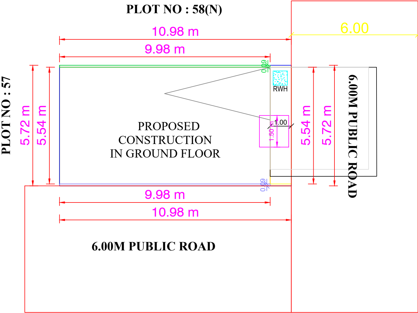
SITE PLAN
