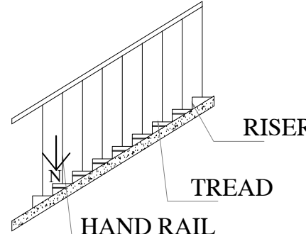
SECTION OF STAIR CASE DETAILS
