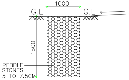
SECTION OF PEBBLE TRENCH SCALE : 1 : = 100
