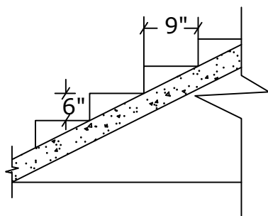
Staircase Detail Not To Scale
