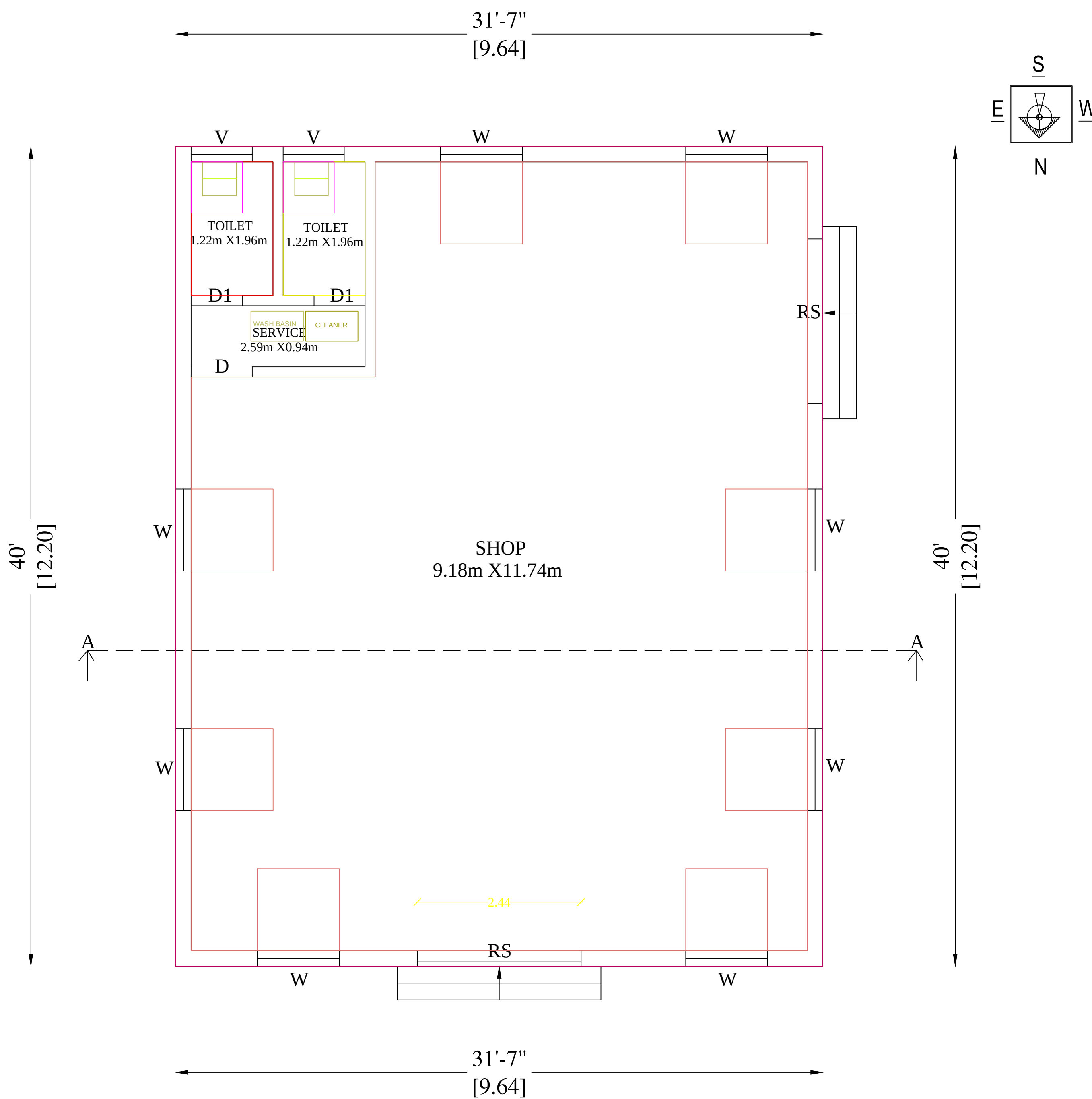
PRO. GROUND FLOOR PLAN
