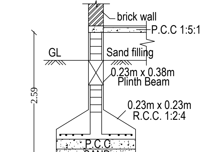
FOUNDATION DETAILS
