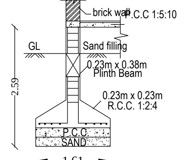
FOUNDATION DETAILS
