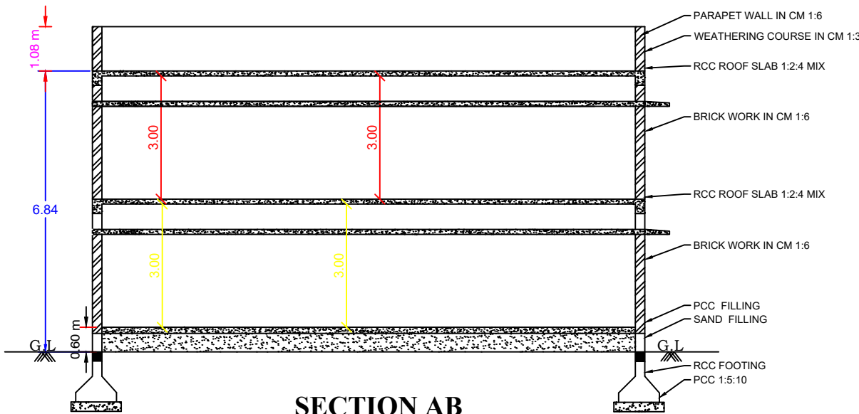
SECTION AB
