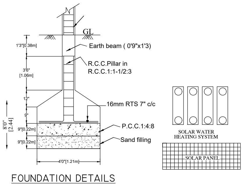
FOUNDATION DETAILS
