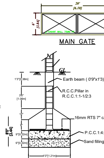
FOUNDATION DETAILS
