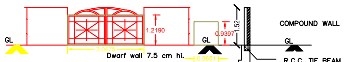
COMPOUND WALL DETAILS
