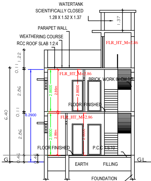
SECTION "A-B"
