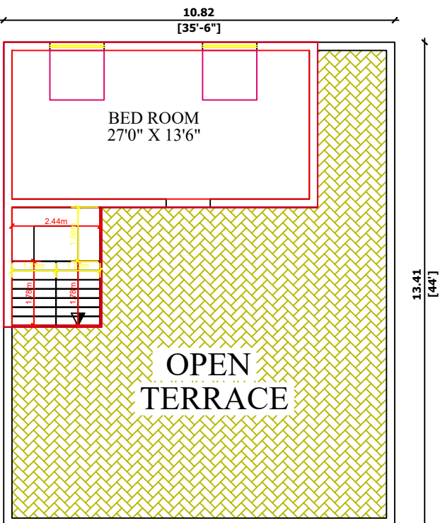
PRO. SECOND FLOOR PLAN.
