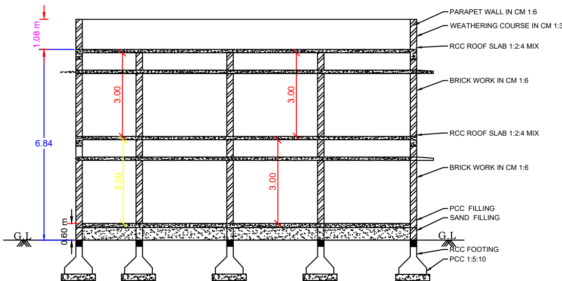
SECTION AB
