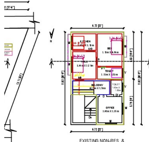
EXISTING NON-RES & PROPOSED RES FIRST FLOOR PLAN
