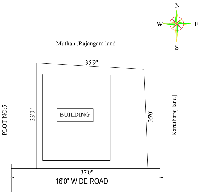
SITE PLAN
