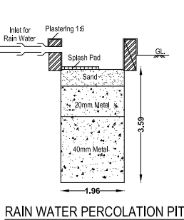
RAIN WATER PERCOLATION PIT
