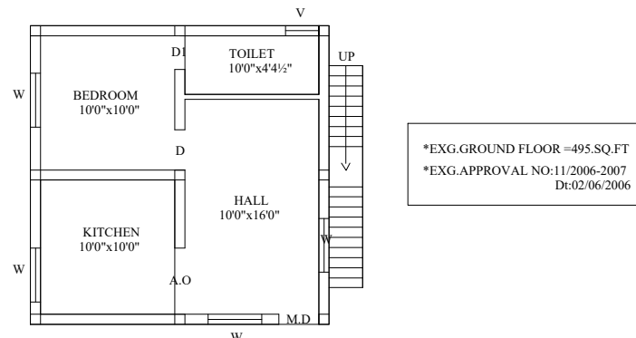
EXG.GROUND FLOOR AREA
