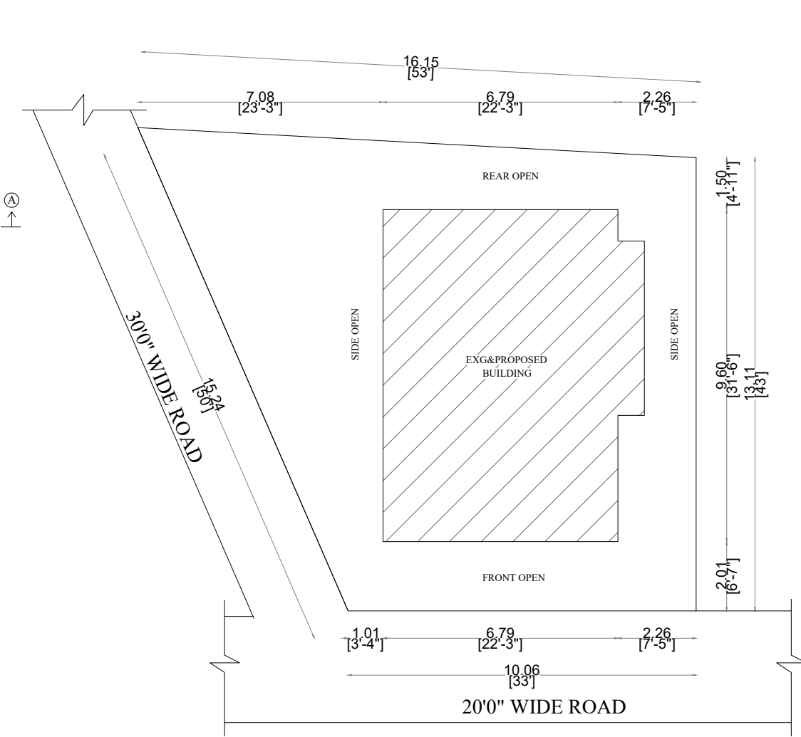
SITE PLAN
