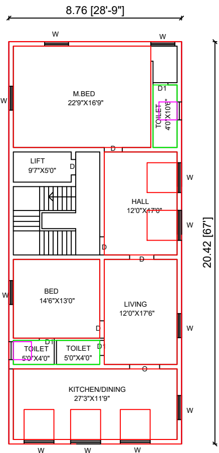
PRO.RESIDENTIAL SECOND FLOOR PLAN
