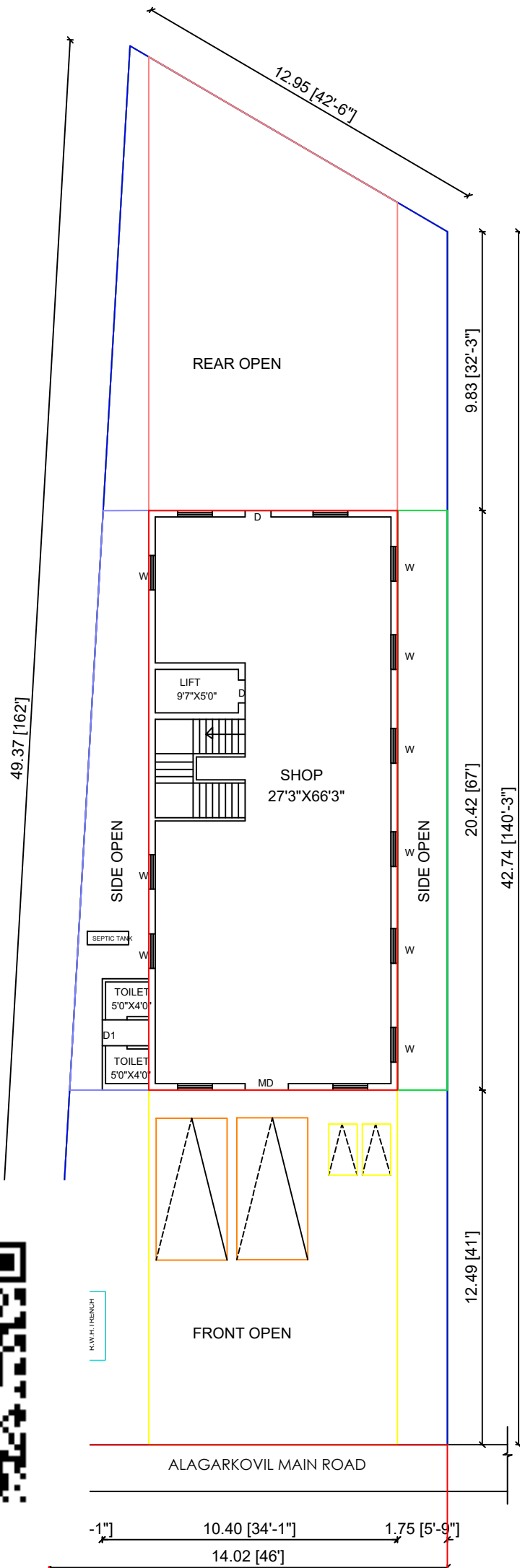
EXG.COMMERCIAL GROUND FLOOR PLAN
