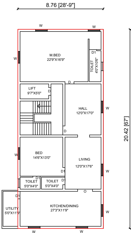
EXG.RESIDENTIAL FIRST FLOOR PLAN
