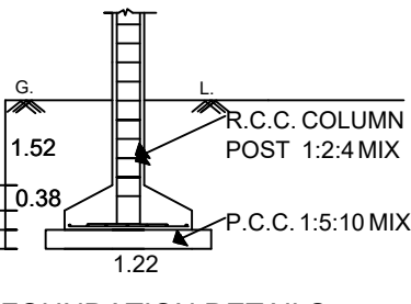
FOUNDATION DETAILS
