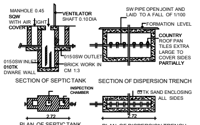
DRAWING FOR SEPTIC TANK WITH DISPERSION TRENCH
