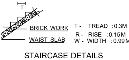
STAIRCASE DETAILS
