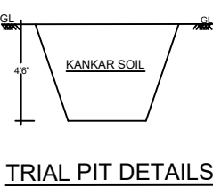
TRIAL PIT DETAILS
