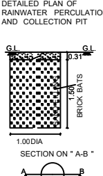
DETAILED PLAN OF RAINWATER PERCOLATION AND COLLECTION PIT
