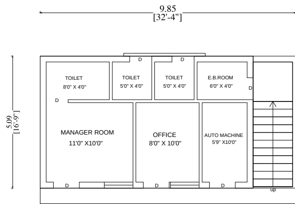
GROUND FLOOR PLAN PROPOSED
