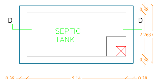
PLAN OF SEPTIC TANK SCALE 1"=2'0"
