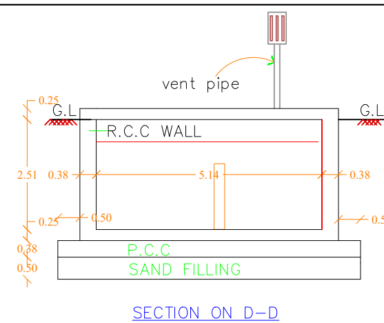
SECTION ON D-D
